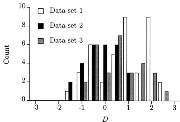
Figure 2 Distribution of Tajima's (1989) D among SDIs, in each of the three data sets.
