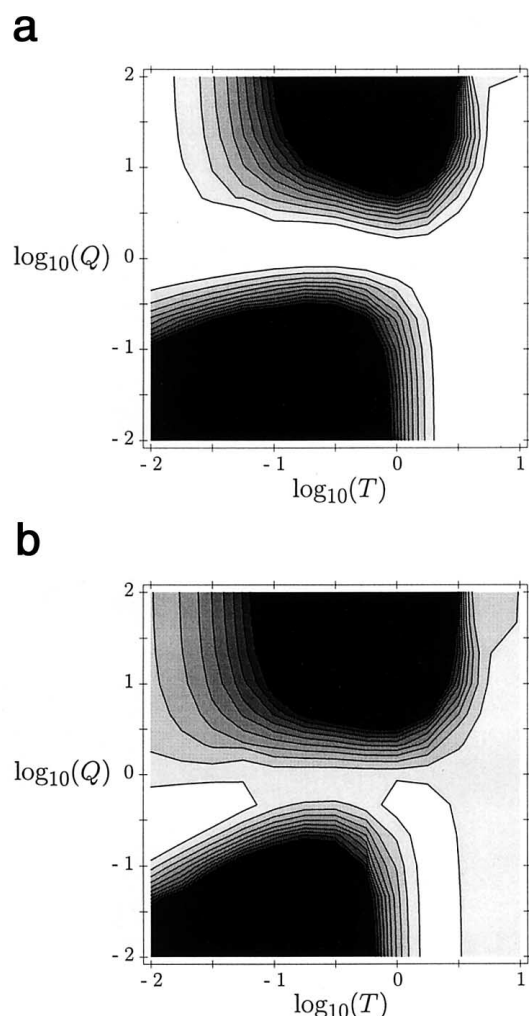
Figure 9 Combined likelihood surfaces for Q and T , for all the data, (a) when the population is assumed to be panmictic and (b) fitting the subdivided-population model described in the text.
