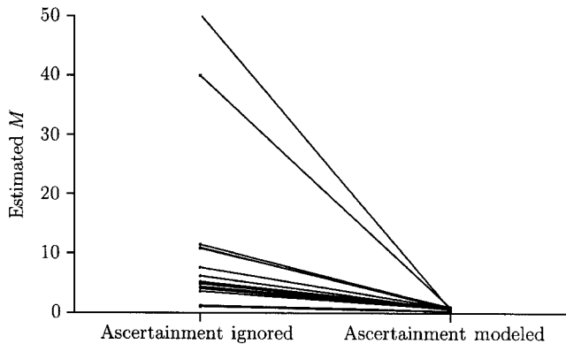
Figure 5 Estimates of 2Nm , for data set 2, both when ascertainment is ignored and when it is modeled. For this data set, five demes had infinite-migration-rate estimates when ascertainment was ignored; these five demes are not plotted.
