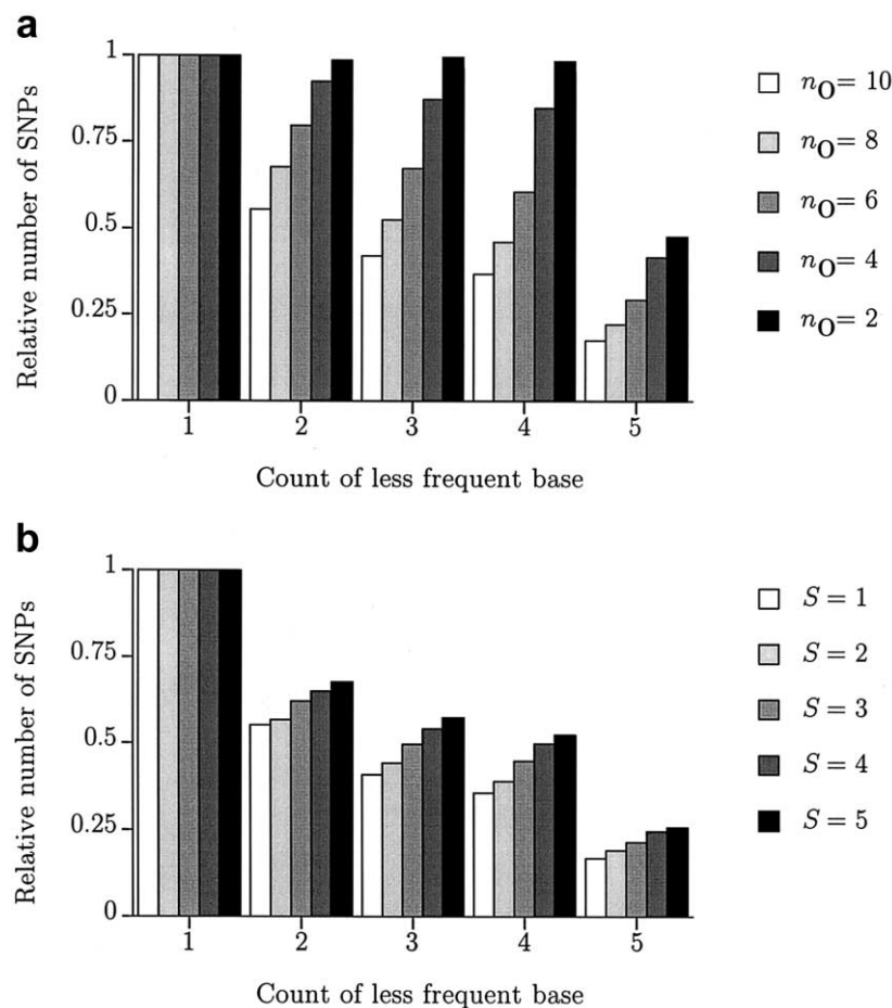
Figure 3 Expected numbers of SNPs segregating in different frequencies, in a sample of size n_D + n_O = 10 , relative to the number of singleton polymorphisms; results are averages, over 100,000 simulated data sets, for a 400-bp-long SDL, with \theta = .0005 per base pair. a , Effect of requiring an SDL to have at least one SNP in the first n_O samples drawn from the population. b , Effect of separating SDLs into classes with different numbers of SNPs, with n_D = 0 .
