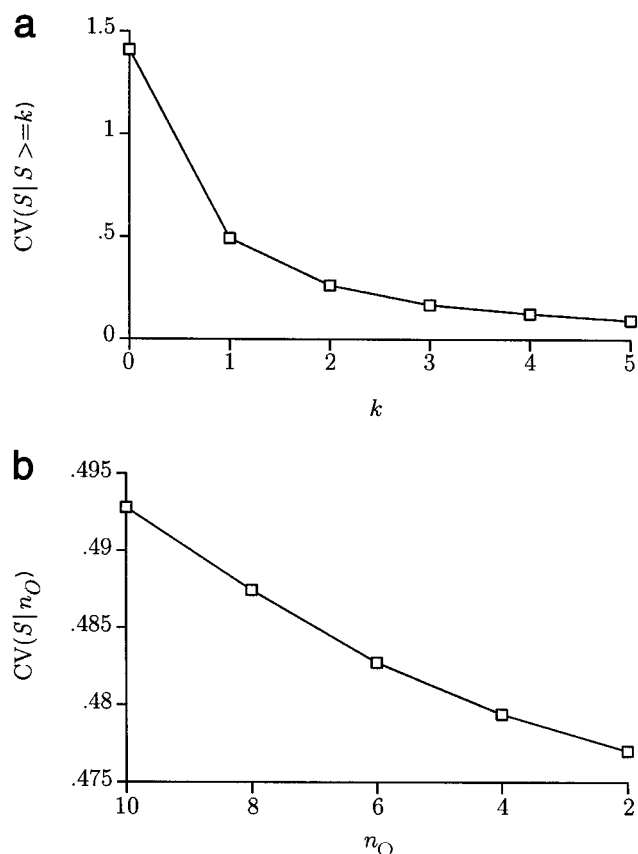
Figure 4 Coefficient of variation of S , in a sample of size n_D + n_O = 10 ; results are averages, over 100,000 simulated data sets, for a 400-bp-long SDL, with \theta = .0005 per base pair. a , Effect of requiring SDLs to have at least k SNPs, under the assumption n_D = 0 . b , Effect of requiring an SDL to have at least one SNP that must be segregating in the first n_O samples drawn from the population.
