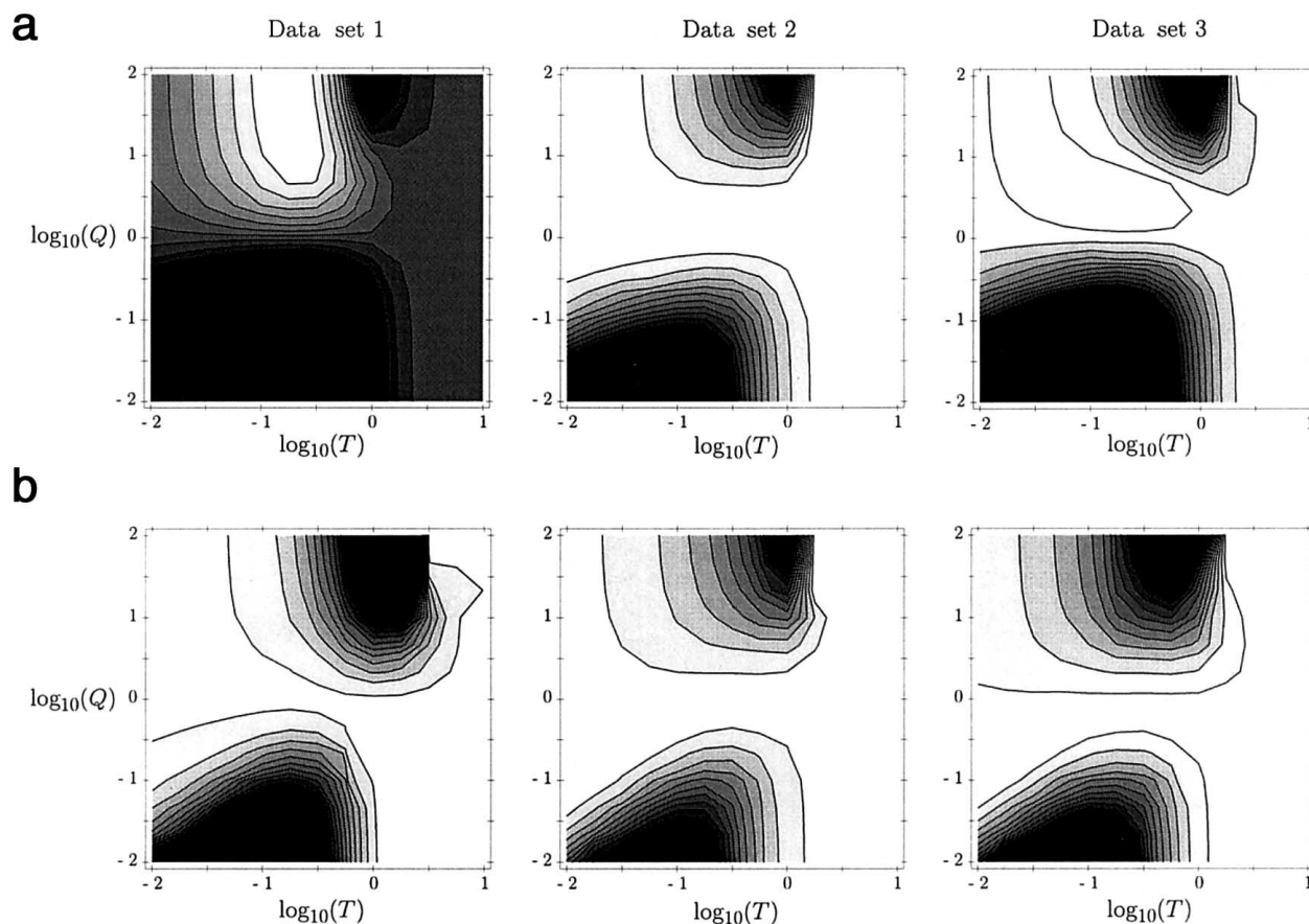
Figure 8 Likelihood surfaces for Q and T , based on the allele frequencies at data-only and overlap SNPs, conditioned on their numbers, for each of the three data sets, when ascertainment bias is ignored (a) and when it is modeled (b).
