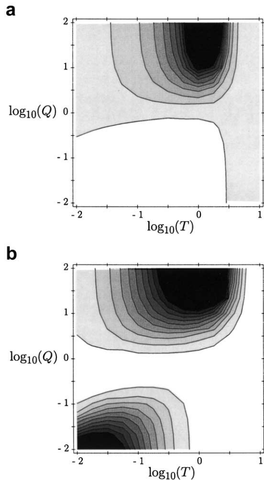
Figure 7 Combined likelihood surfaces for Q and T , based on the distribution of n_D and n_O for all three data sets, when ascertainment bias is ignored (a) and when it is modeled (b).
