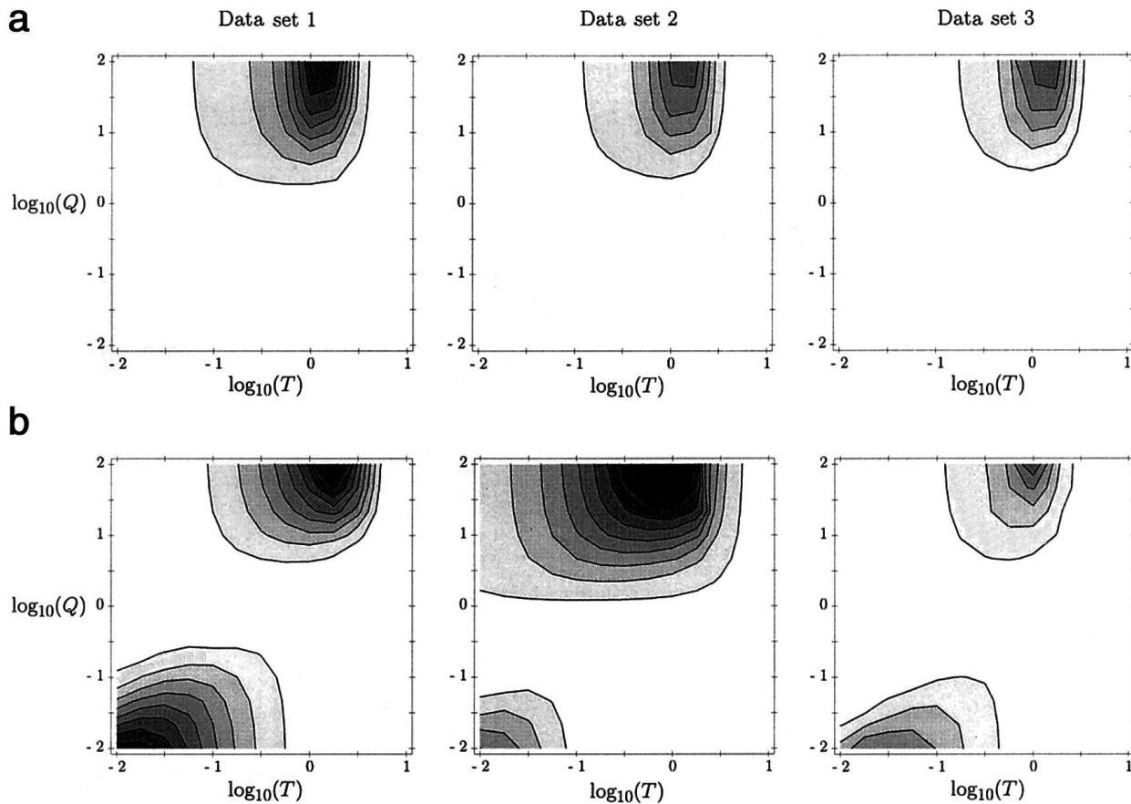
Figure 6 Likelihood surfaces for Q and T , based on the distribution of n_D and n_O for each of the three data sets, when ascertainment bias is ignored (a) and when it is modeled (b).
